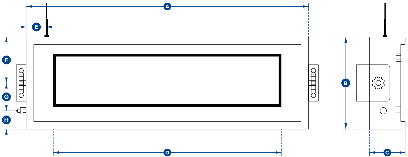
Front Elevation
